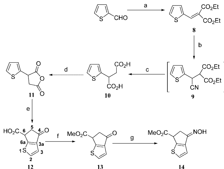
Scheme 1. (a) Diethyl malonate, piperidine, toluene, reflux; (b) KCN/H 2 O, EtOH, reflux (c) (1) 1.5 N NaOH, reflux; (2) 6 M HCl, reflux; (d) AcCl, reflux; (e) AlCl 3 , 1,2-dichloroethane, room temp.; (f) MeOH, TsOH, reflux; (g) NH 2 OH·HCl, NaAc/H 2 O, EtOH, reflux.
