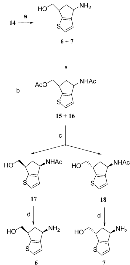
Scheme 2. (a) AlH 3 , THF, reflux; (b) Ac 2 O, Et 3 N, room temp.; (c) (1) K 2 CO 3 , MeOH, room temp.; (2) flash chromatography; (d) (1) 2 M HCl, MeOH, reflux; (2) Amberlite IRA-400 (OH).
